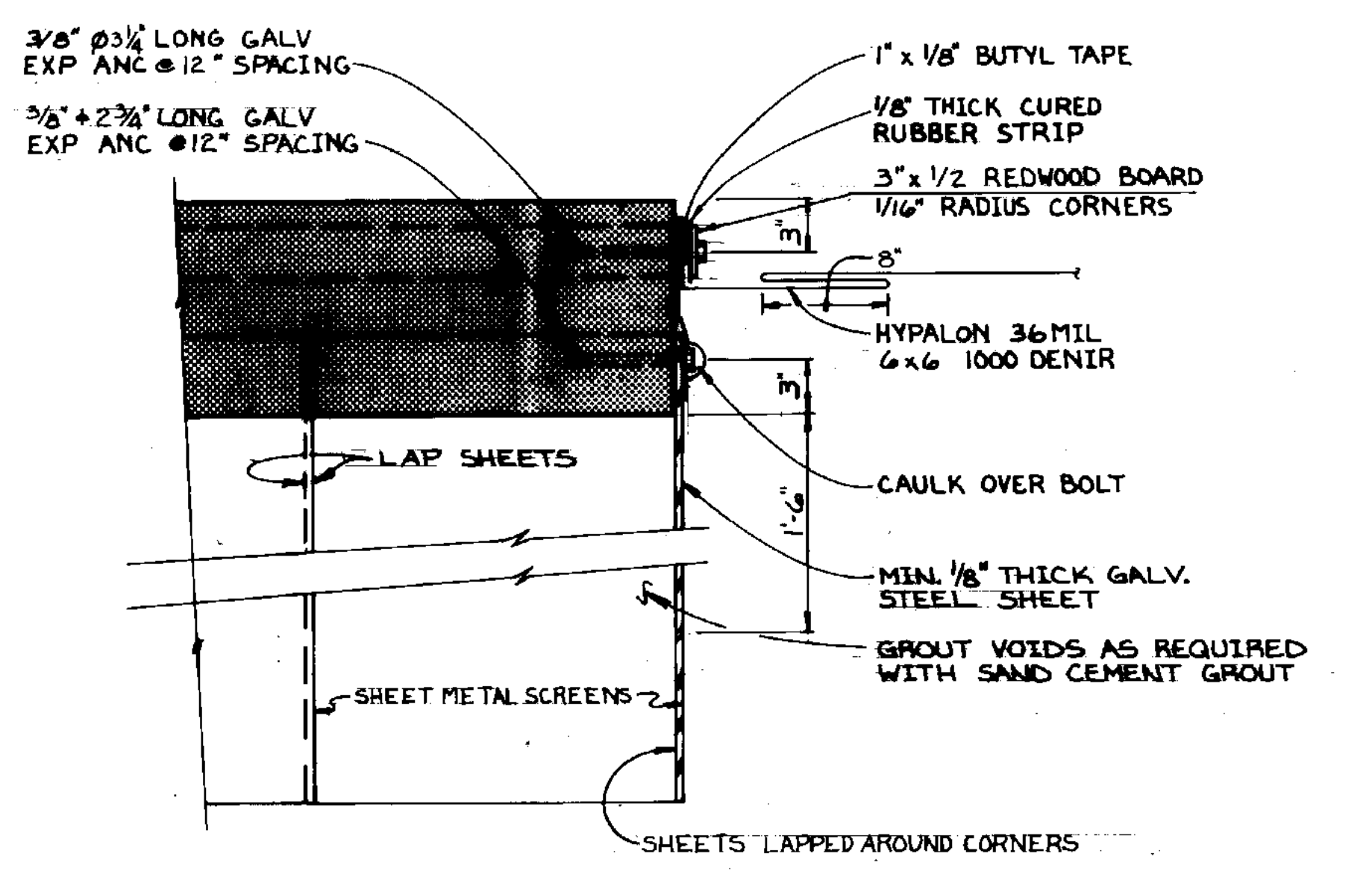
DETAIL A NO SCALE SEE THIS DWG.
